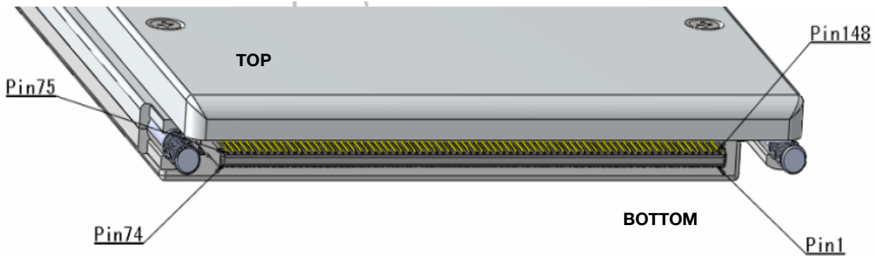
Figure 2. Transceiver Electrical Pad Layout
