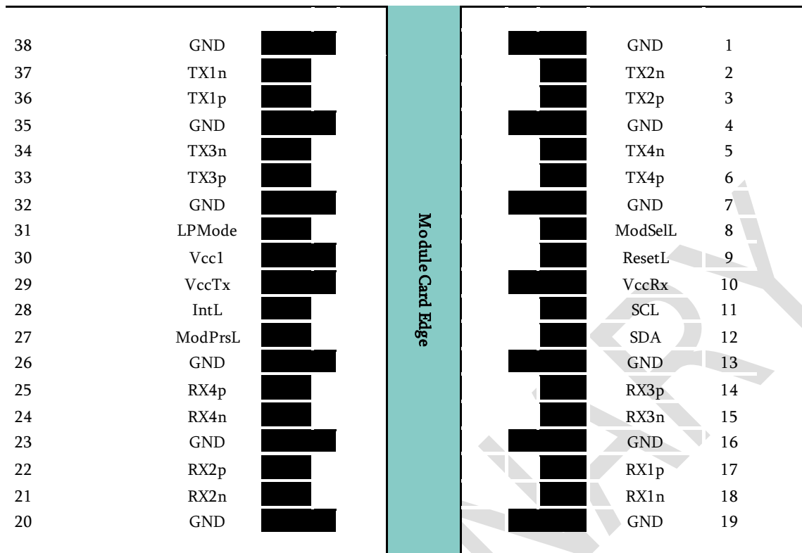
Figure 2. QSFP28 Module Pad Layout
