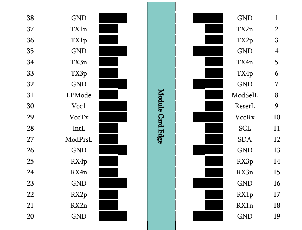
Figure 2. QSFP28 Electrical Pad Layout
