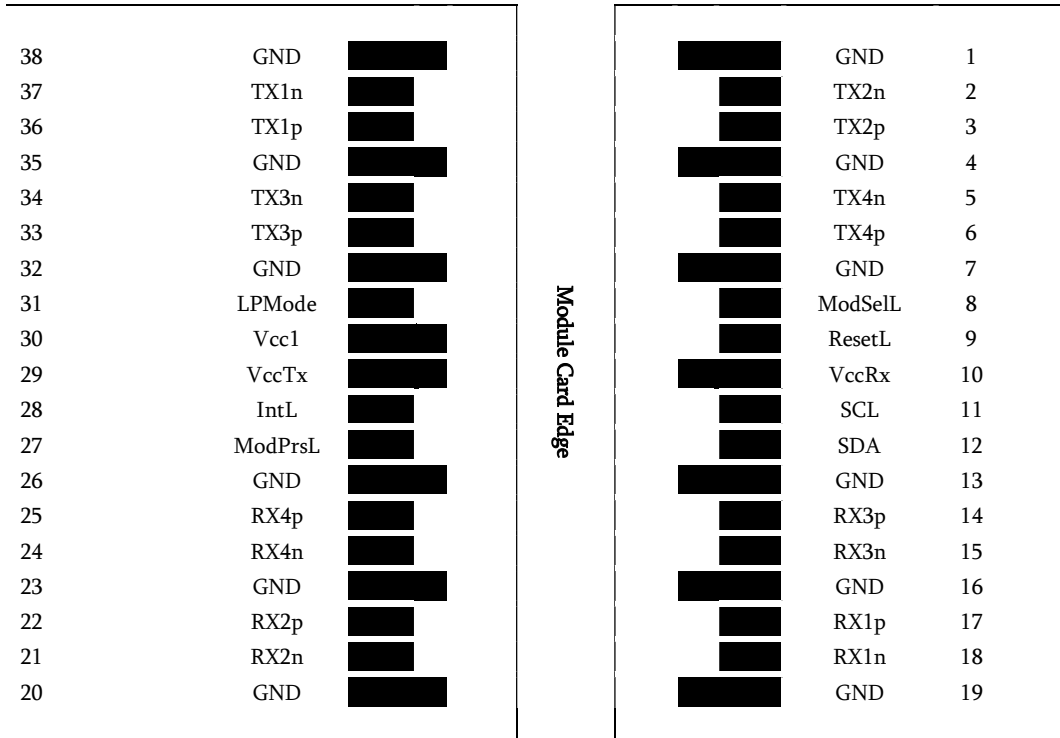
Figure 2. QSFP+ Module Pad Layout
