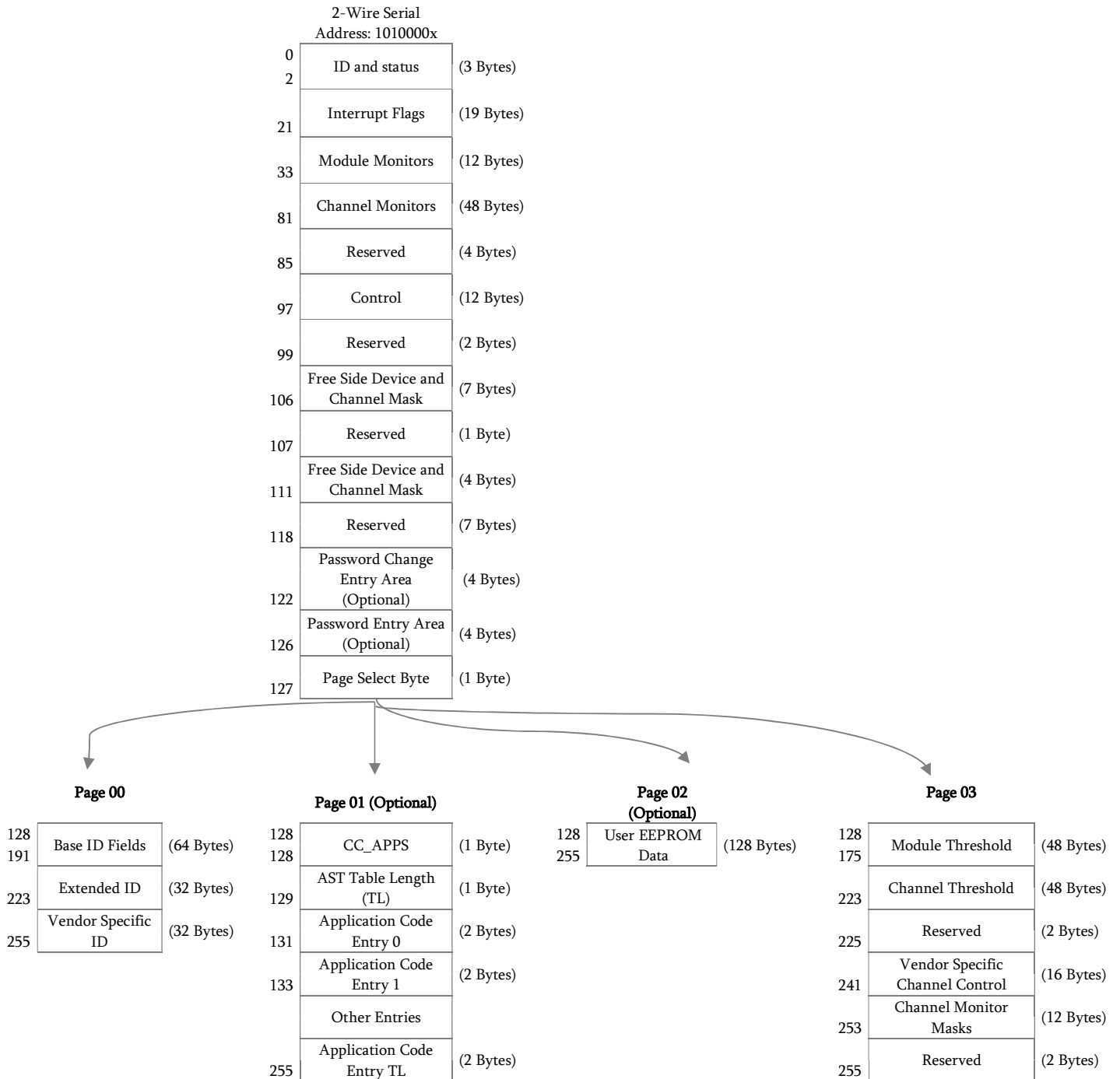
Figure 3. QSFP+ Memory Map
