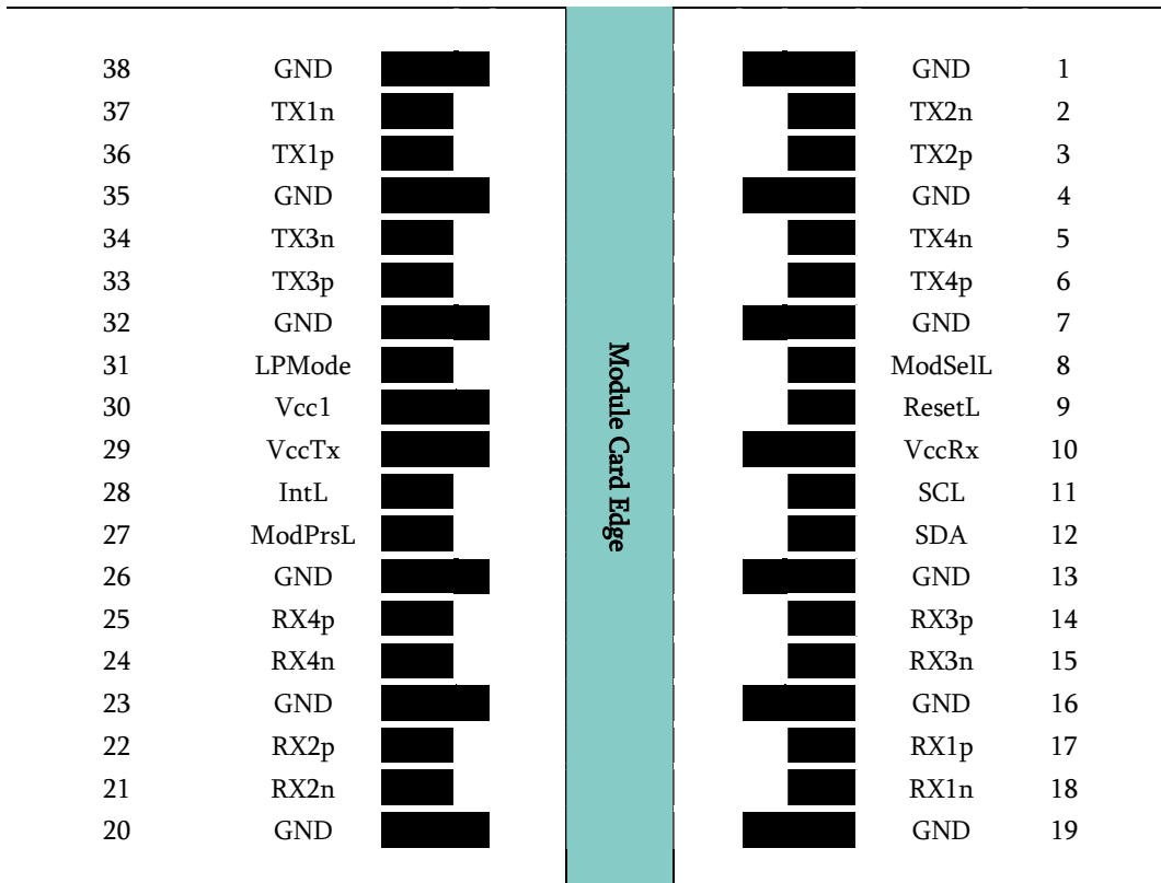
Figure 2. QSF28 Electrical Pad Layout
