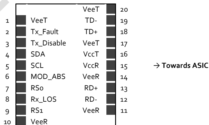
Figure 2. Transceiver Electrical Pad Layout
