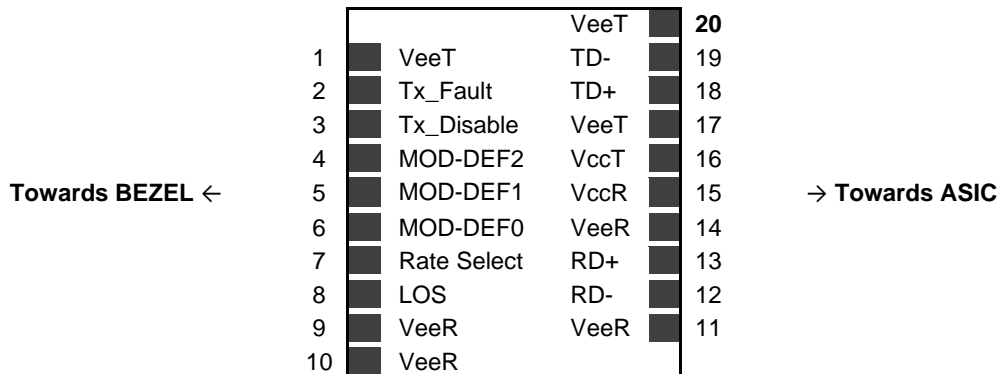
Figure 2. Transceiver Electrical Pad Layout
