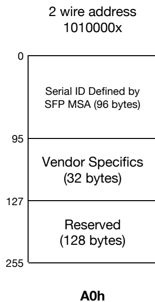
Figure 3. EEPROM of a SFP
