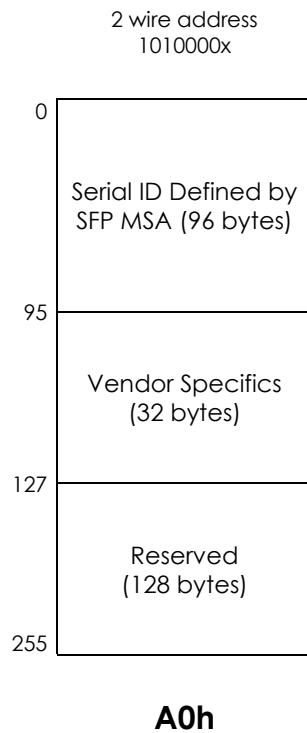
Figure 3. EEPROM of a SFP Copper
