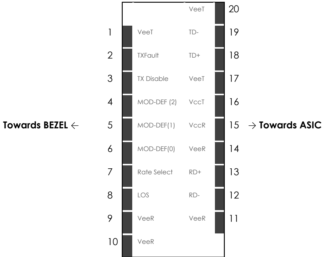
Figure 2. Transceiver Electrical Pad Layout
