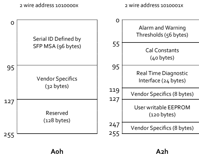
Figure 3. SFP+ Memory Map
