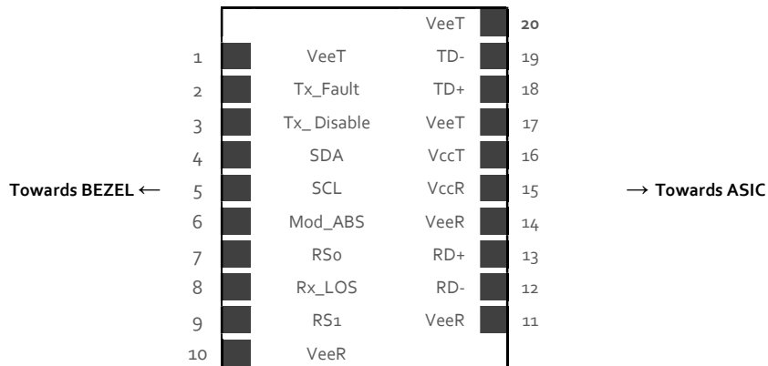
Figure 2. Transceiver Electrical Pad Layout
