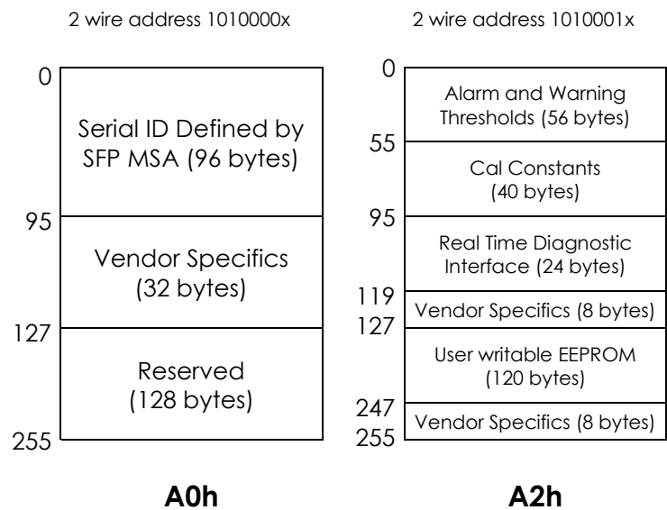
Figure 3. EEPROM of a SFP+
