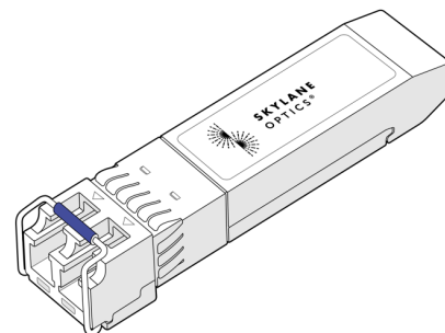
Figure 1. SFP+ Dual Fibre (non-binding illustration)
