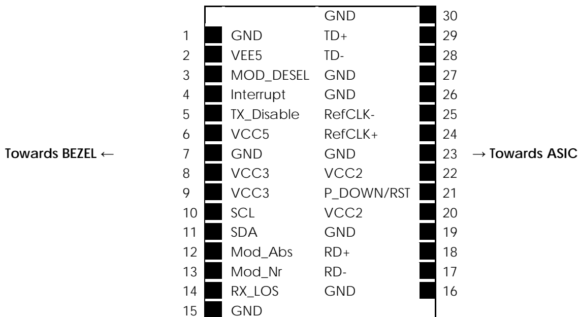
Figure 2. Transceiver Electrical Pad Layout
